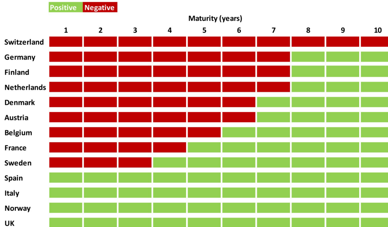
Negative rates in European government bond markets
